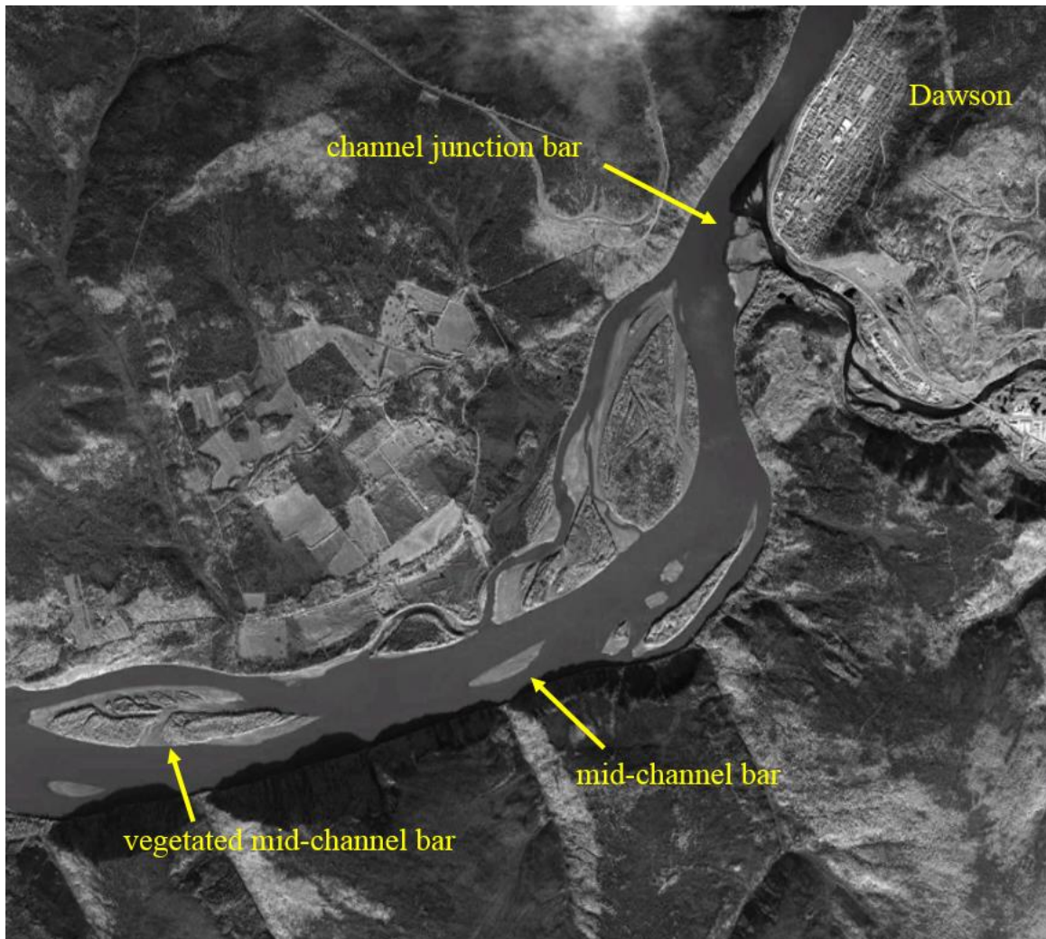
Figure 15: Examples of channel bars in vicinity of Dawson, YK. Base image obtained from Google Earth.
