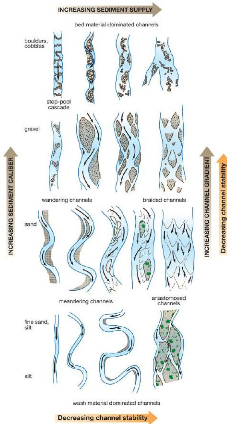
Figure A1: Examples of alluvial channel forms [22].
